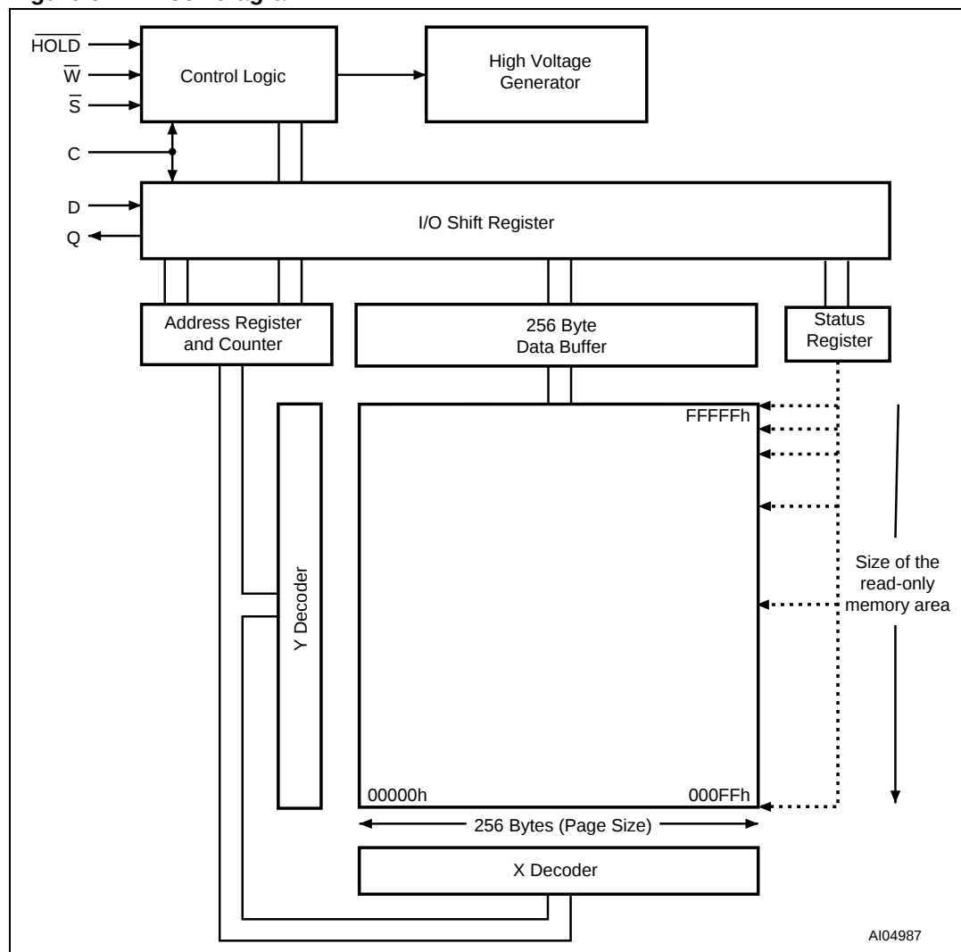
Figure 6. Block diagram
